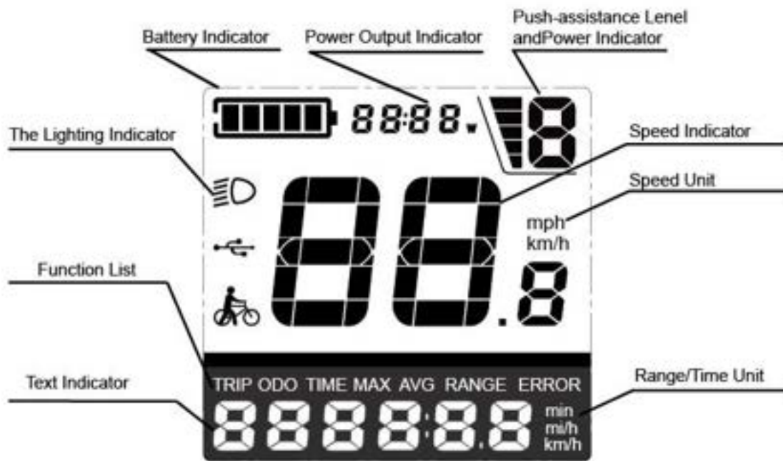
Functional Area Distribution
